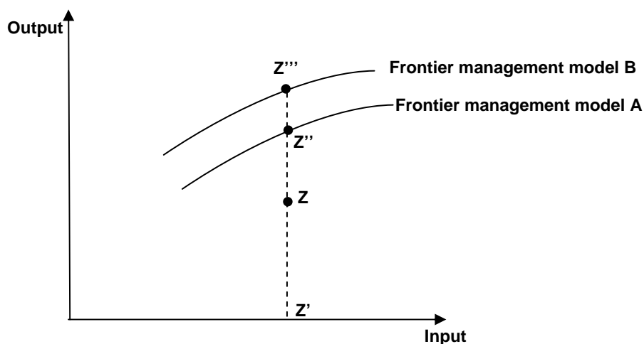
Figure 1. Efficiency decomposition according to Silva Portela & Thanassoulis (2001)
